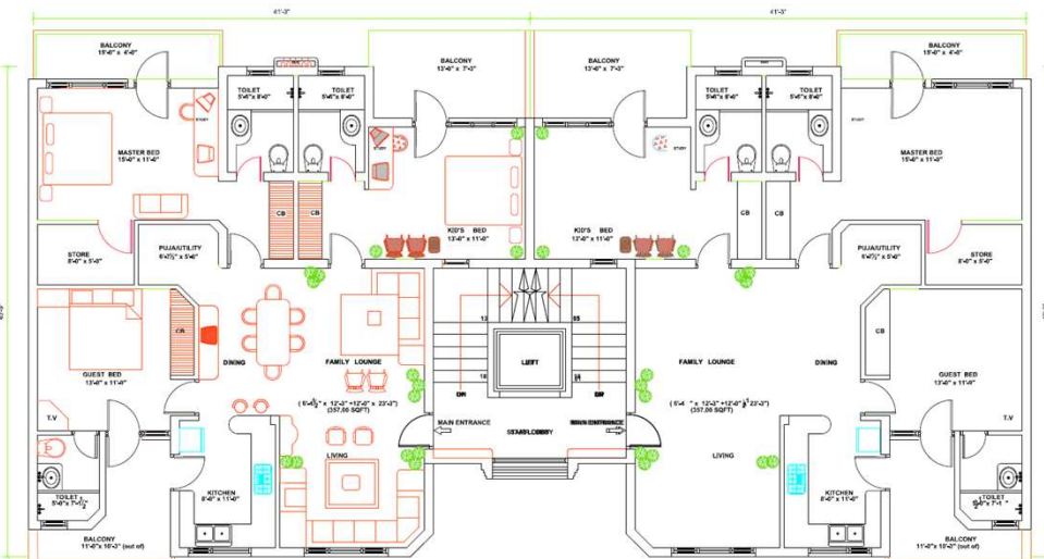
TYPICAL FLOOR PLAN THREE BED ROOM WITH THREE TOILETS TOTAL COVERED AREA ■ 1665 SQFT
