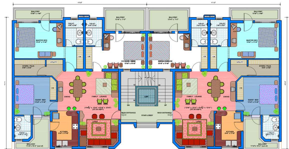
TYPICAL FLOOR PLAN THREE BED ROOM WITH THREE TOILETS TOTAL COVERED AREA ■ 1350.00 SQFT
